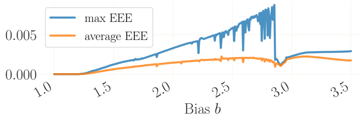
Figure B.14: Average and maximum absolute Euler equation errors for the simulations in Figure 6 when using policy function iteration.
