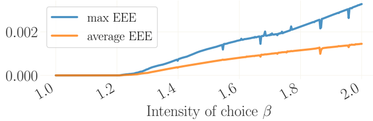
Figure B.12: Average and maximum absolute Euler equation errors for the simulations in Figure 2 when using policy function iteration.
