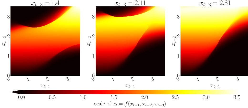
Figure 10: Heatmap for slices of the policy function g for the chaotic time series in Figure 9. The mapping of f is nontrivial and not smooth on the relevant domain. For this figure we use the policy function iteration method outlined in Appendix A with a grid of 300 \times 300 \times 300 points to obtain a high resolution of the image. Note that for the dynamics of the time series this increase in precision is not relevant.
