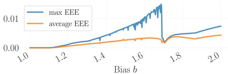
Figure B.13: Average and maximum absolute Euler equation errors for the simulations in Figure 3 when using policy function iteration.
