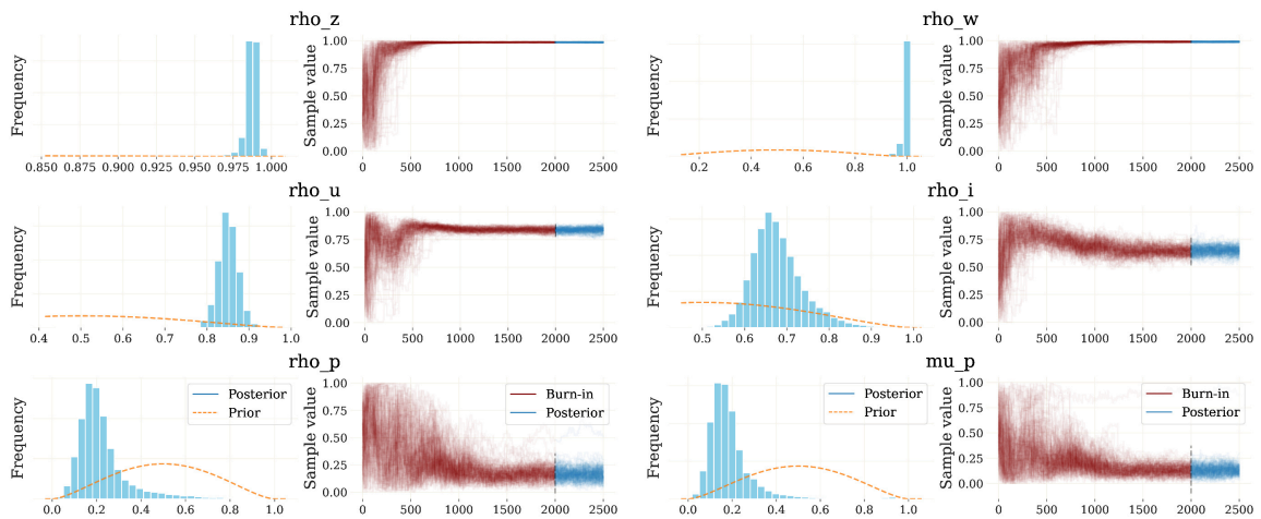
Figure E.11: Traceplots of the 200 ADEMC chains for selected parameters. Estimation of the benchmark model. The left panel shows a KDE of the parameter distribution. The right displays the trace of each of the chains over time.
