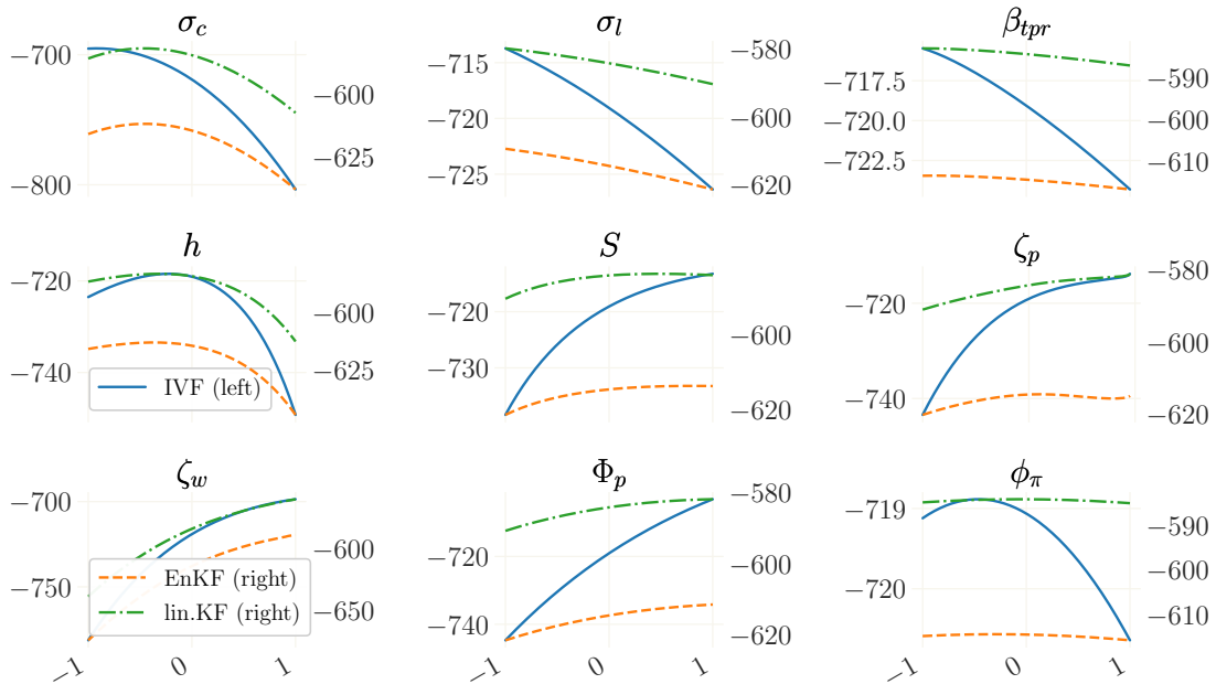
Figure D.6: Likelihood evaluations for an artificial dataset without binding ELB. For each panel, all parameters are set to the prior mean while one parameter is varied within one standard deviation of its prior distribution (x-axis). Left y-axis: likelihood evaluations with the IVF; right y-axis: likelihood evaluations with the EnKF and the KF.
