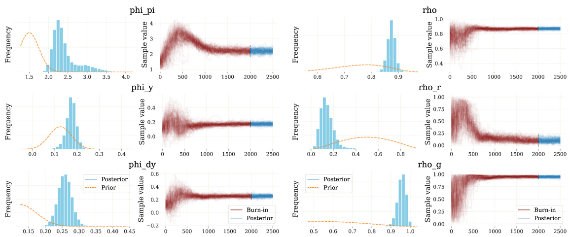
Figure E.10: Traceplots of the 200 ADEMC chains for selected parameters. Estimation of the benchmark model. The left panel shows a KDE of the parameter distribution. The right displays the trace of each of the chains over time.
