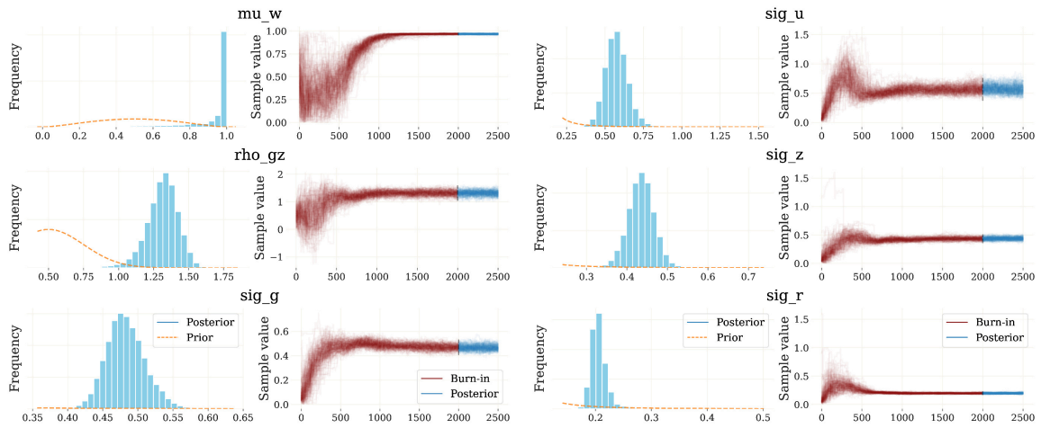
Figure E.12: Traceplots of the 200 ADEMC chains for selected parameters. Estimation of the benchmark model. The left panel shows a KDE of the parameter distribution. The right displays the trace of each of the chains over time.
