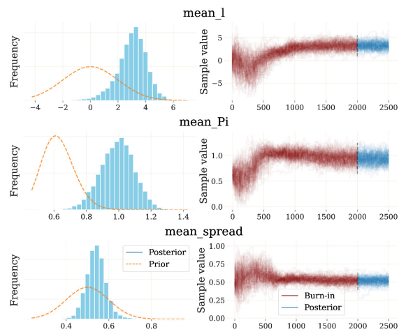
Figure E.14: Traceplots of the 200 ADEMCM chains for selected parameters. Estimation of the benchmark model. The left panel shows a KDE of the parameter distribution. The right displays the trace of each of the chains over time.
