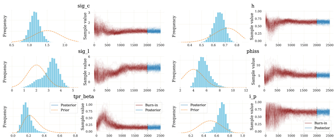
Figure E.8: Traceplots of the 200 ADEMC chains for selected parameters. Estimation of the benchmark model. The left panel shows a KDE of the parameter distribution. The right displays the trace of each of the chains over time.
