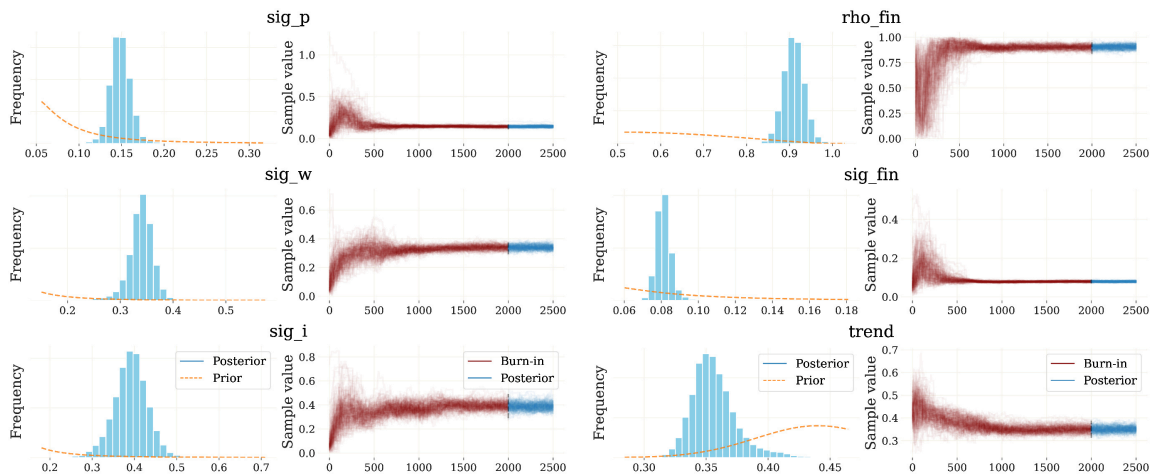
Figure E.13: Traceplots of the 200 ADEMC chains for selected parameters. Estimation of the benchmark model. The left panel shows a KDE of the parameter distribution. The right displays the trace of each of the chains over time.
