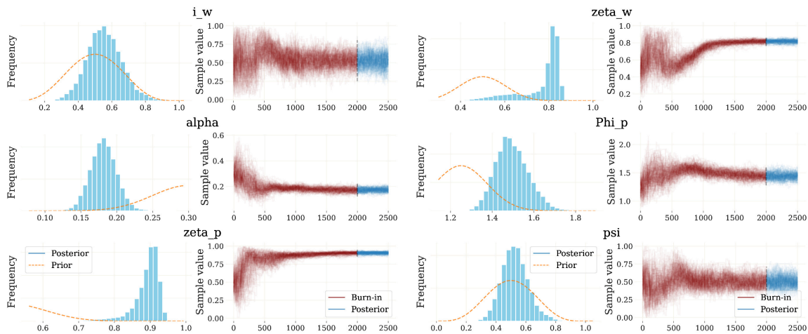
Figure E.9: Traceplots of the 200 ADEMC chains for selected parameters. Estimation of the benchmark model. The left panel shows a KDE of the parameter distribution. The right displays the trace of each of the chains over time.
