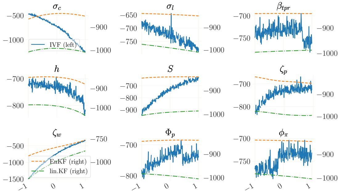
Figure D.7: Likelihood evaluations given for an artificial dataset where the ELB binds for 30 subsequent quarters. For each panel, all parameters are set to the prior mean while one parameter is varied within one standard deviation of its prior distribution (x-axis). Left y-axis: likelihood evaluations with the IVF; right y-axis: likelihood evaluations with the EnKF and the KF.
