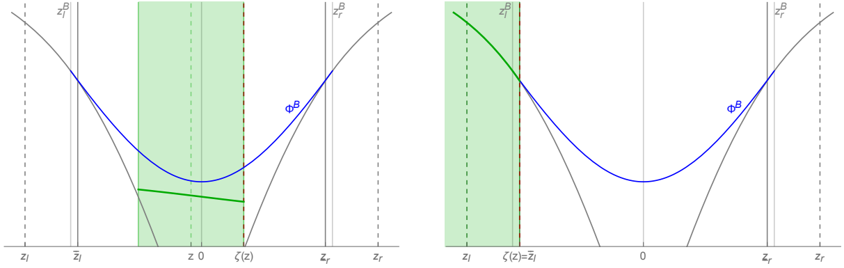
Figure 10: Agent’s value when experimenting (left) and when stopping (right), with worst-case belief \zeta(z) and boundaries \bar{z}_\ell := z_\ell + \Delta/2 and \bar{z}_r := z_r - \Delta/2 . The Bayesian value function is \Phi^B(z) := \phi(z|z_\ell^B, z_r^B) .
